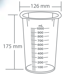
1000 ml Ezipour Measuring Beaker marked with 20 ml graduations
