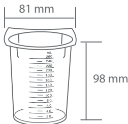
250 ml Ezipour Measuring Beaker marked with 10 ml graduations 10 - 260mL
